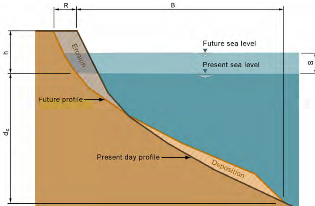
Figure I10: Illustration of variables in the Bruun Rule
