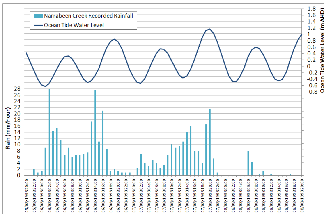
Figure 5-26 August 1998 Recorded Tidal Water Level
