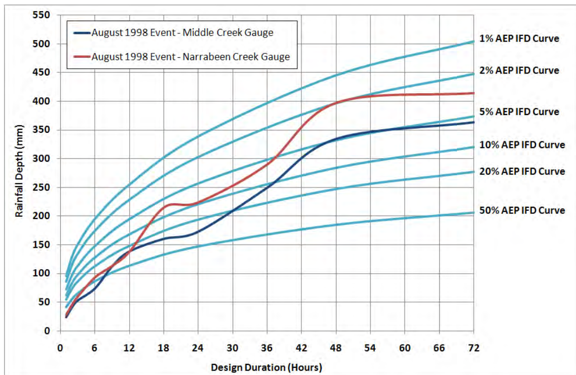
Figure 5-24 Comparison of August 1998 Rainfall with IFD Relationships
