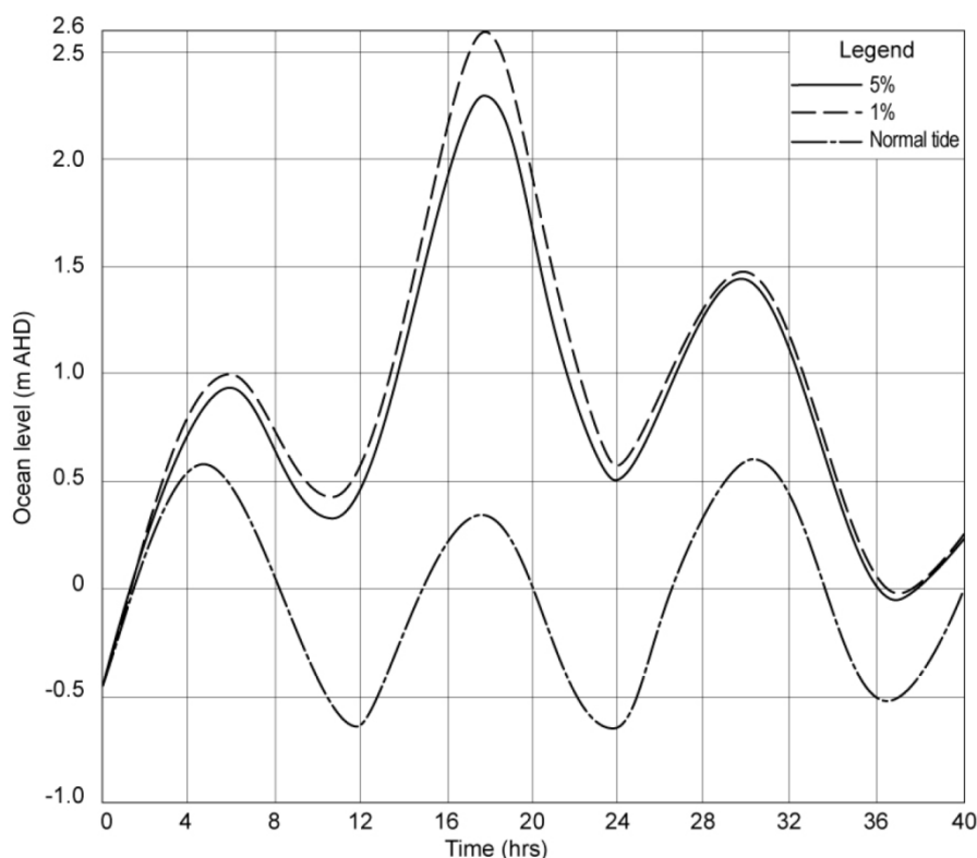
Figure 6-1 DECCW Recommended Design Ocean Boundaries
