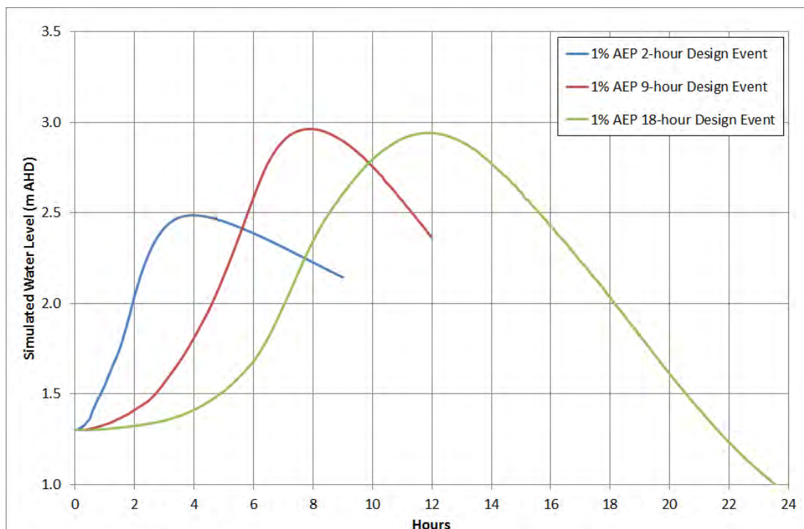
Figure 7-7 Simulated Water Level Response in Narrabeen Lagoon
