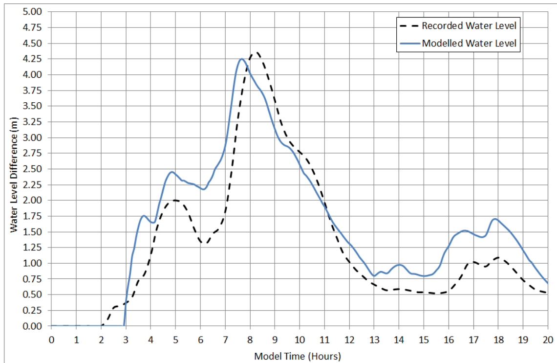
Figure 5-11 Middle Creek Water Level Calibration – April 1998
