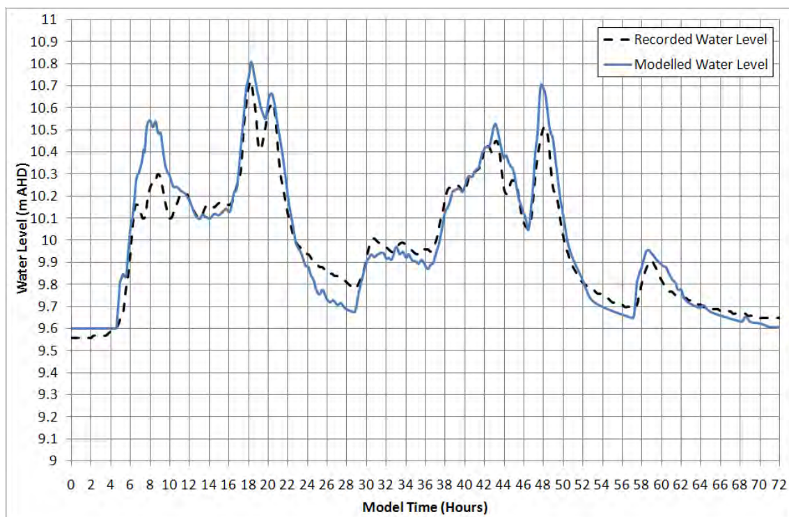
Figure 5-31 Fern Creek Water Level Validation – August 1998
