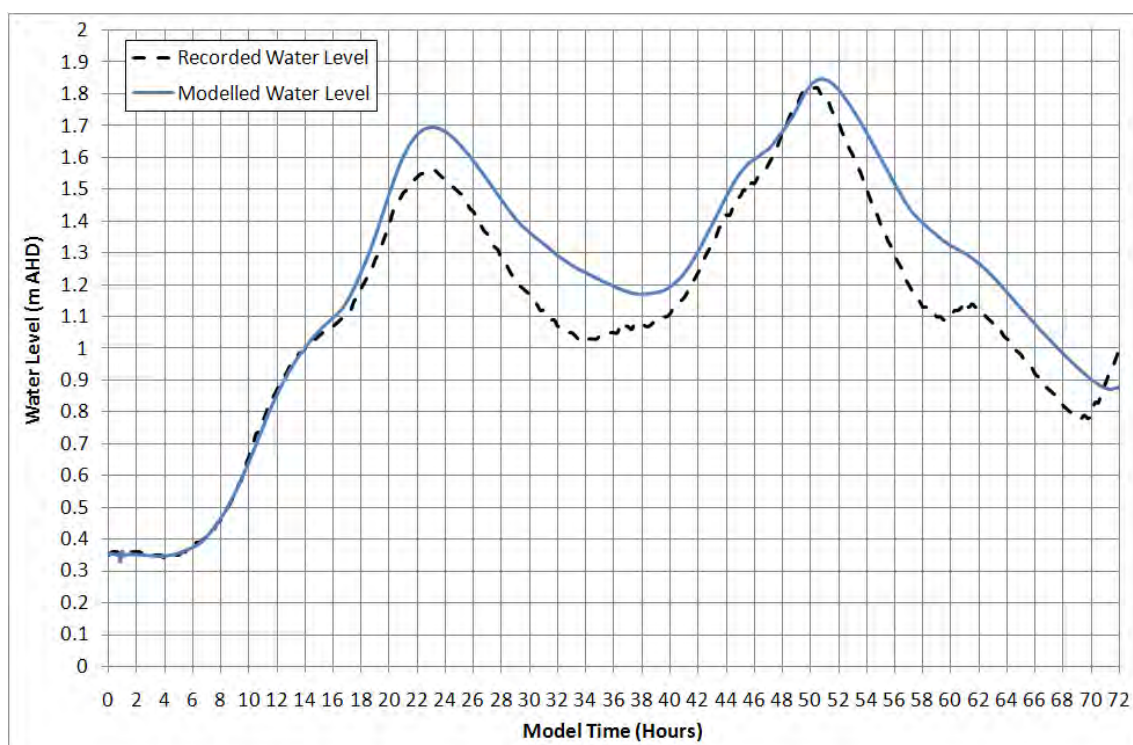
Figure 5-28 Pittwater Road Bridge Water Level Validation – August 1998
