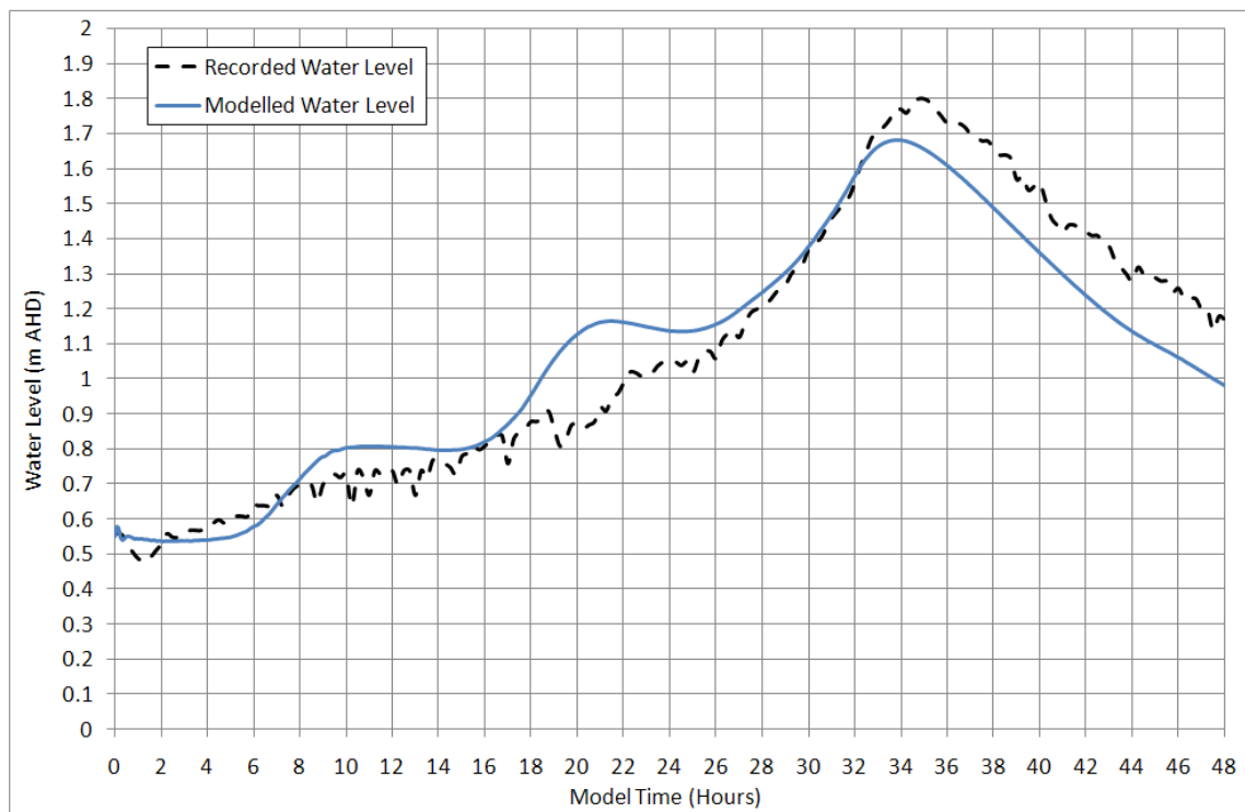
Figure 5-19 Pittwater Road Bridge Water Level Validation – March 2011
