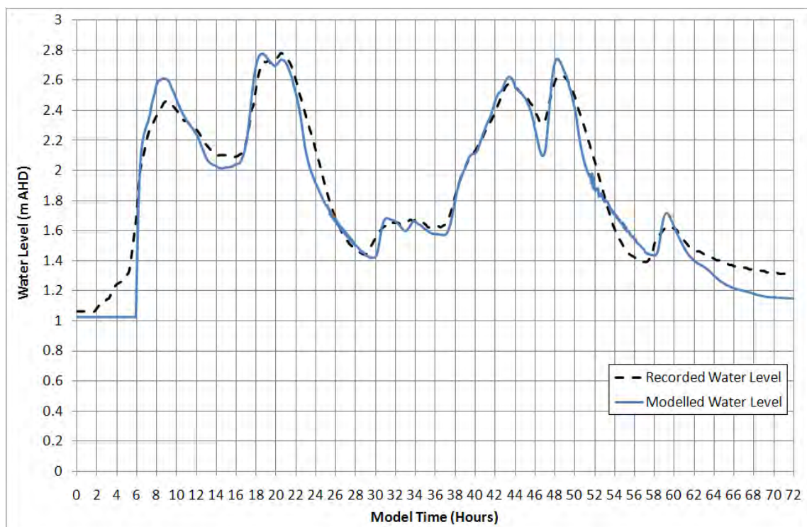
Figure 5-30 Narrabeen Creek Water Level Validation – August 1998
