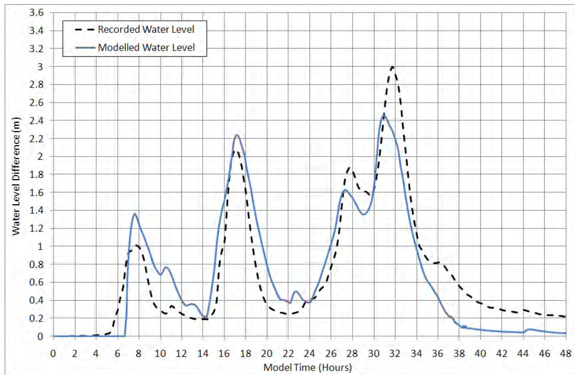
Figure 5-20 Middle Creek Water Level Validation – March 2011
