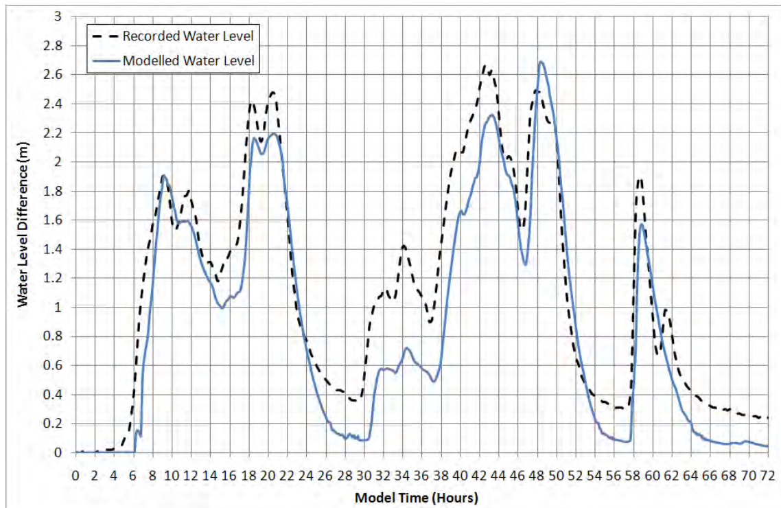
Figure 5-29 Middle Creek Water Level Validation – August 1998
