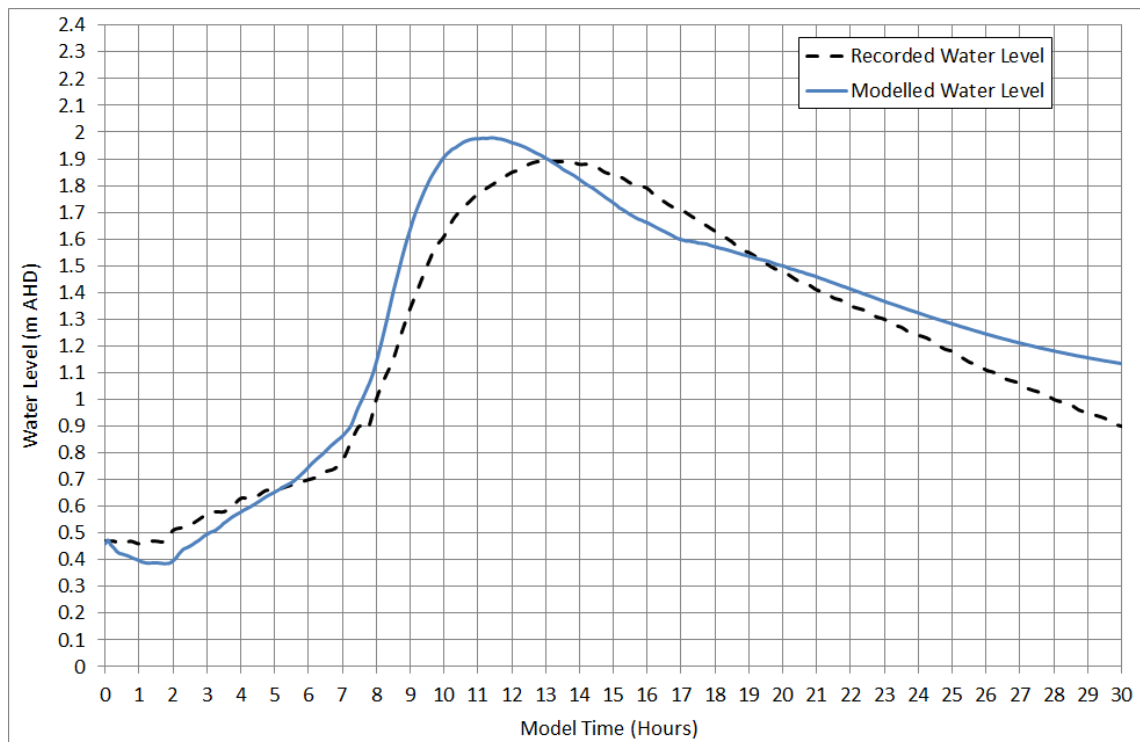
Figure 5-9 Ocean Street Water Level Calibration – April 1998
