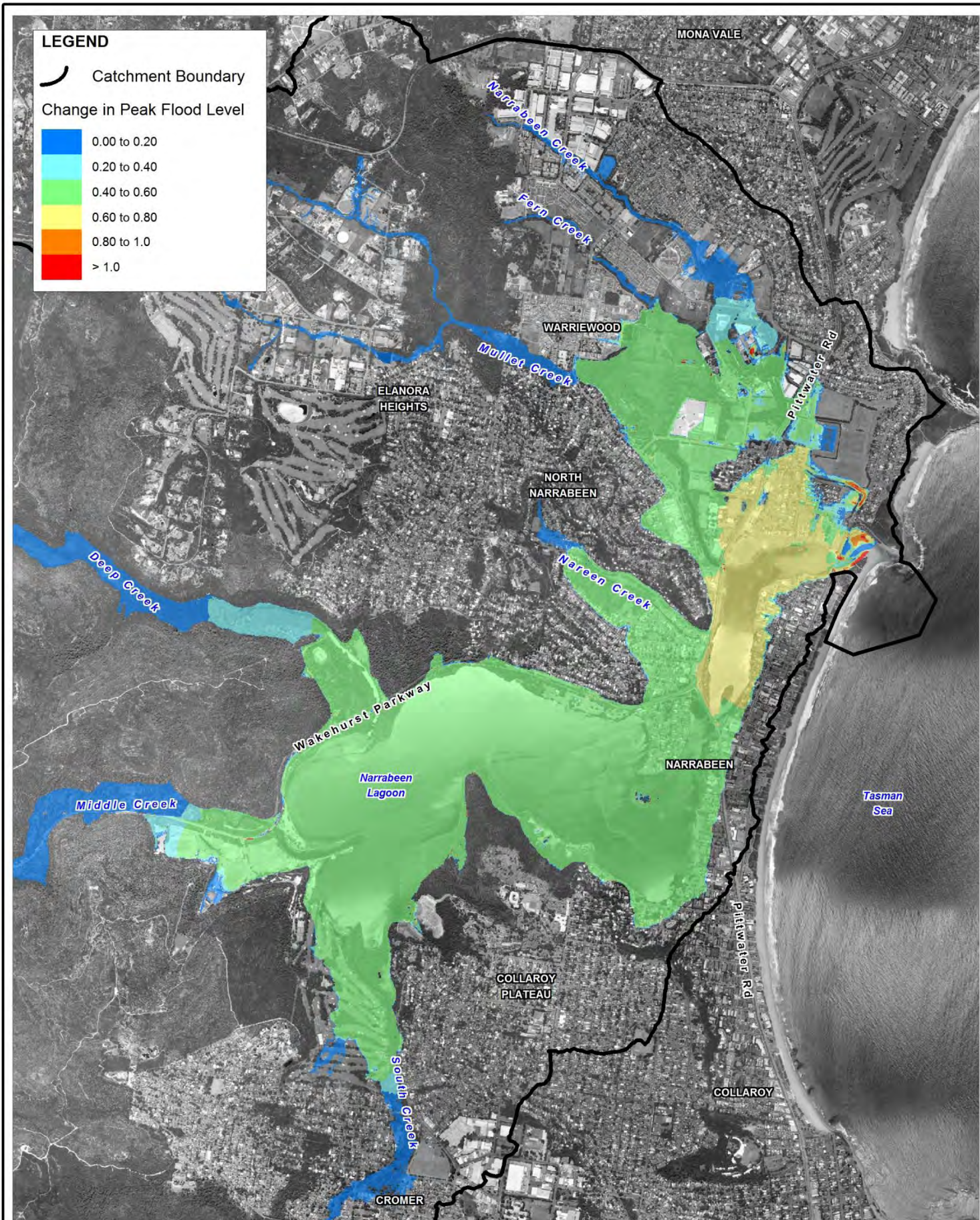
Title: Peak 1% AEP Flood Level Increase with 0.9m Sea Level Rise
