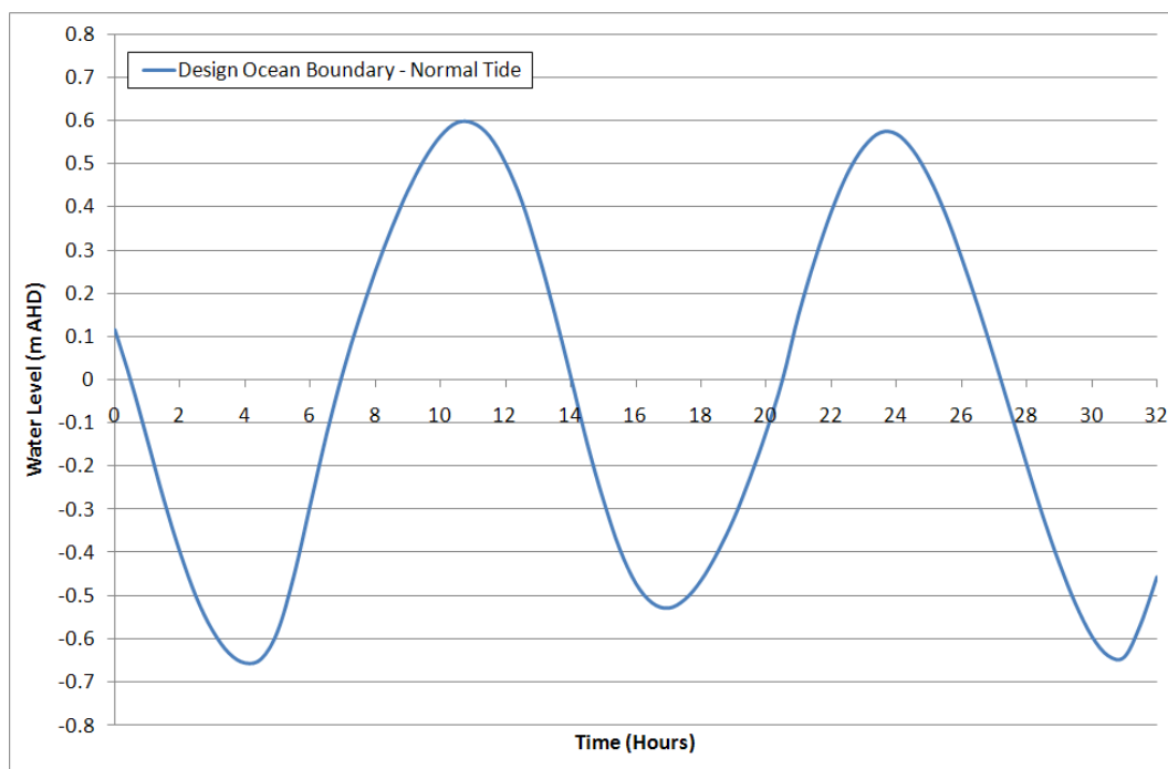
Figure 6-2 Design Ocean Boundary – Normal Tide
