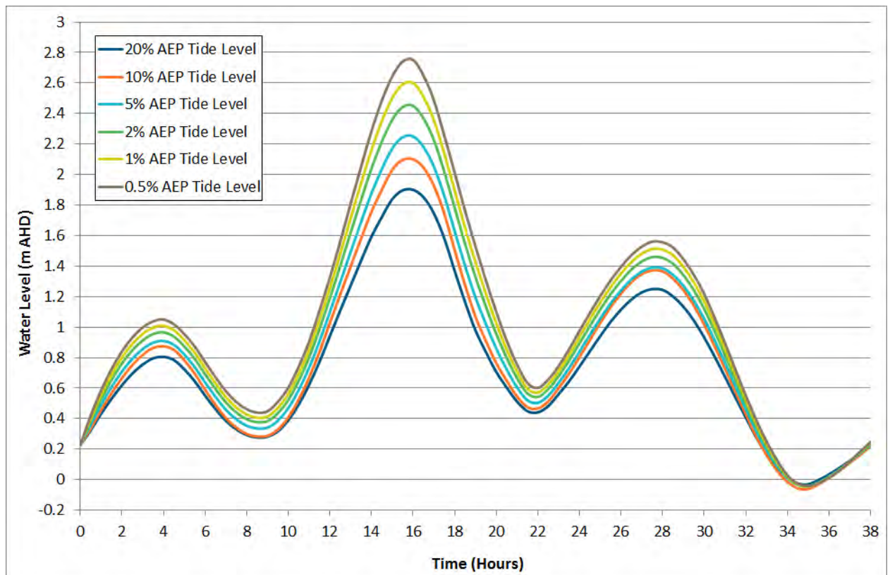
Figure 6-3 Design Ocean Boundary – Elevated Tide
