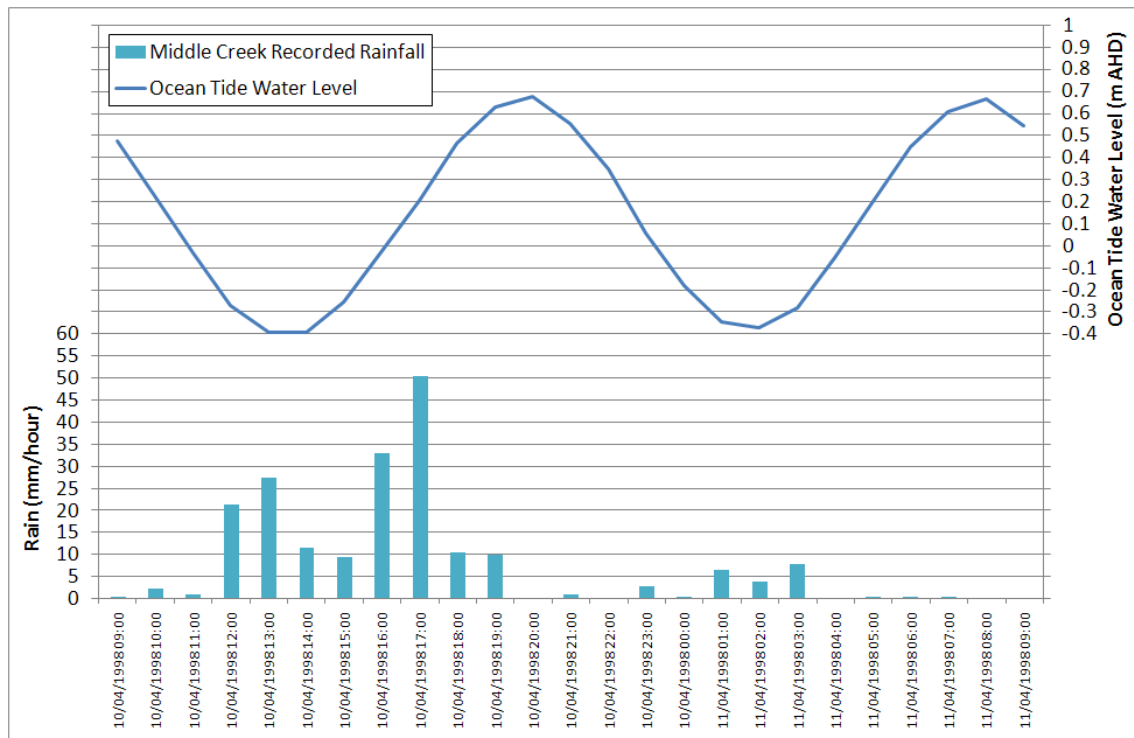
Figure 5-5 April 1998 Recorded Tidal Water Level
