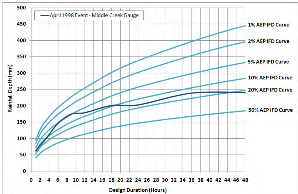
Figure 5-3 Comparison of April 1998 Rainfall with IFD Relationships
