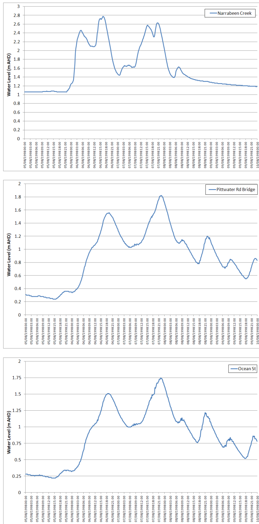
Figure 5-25 August 1998 Recorded Water Levels
