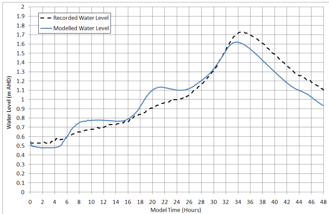
Figure 5-18 Ocean Street Water Level Validation – March 2011
