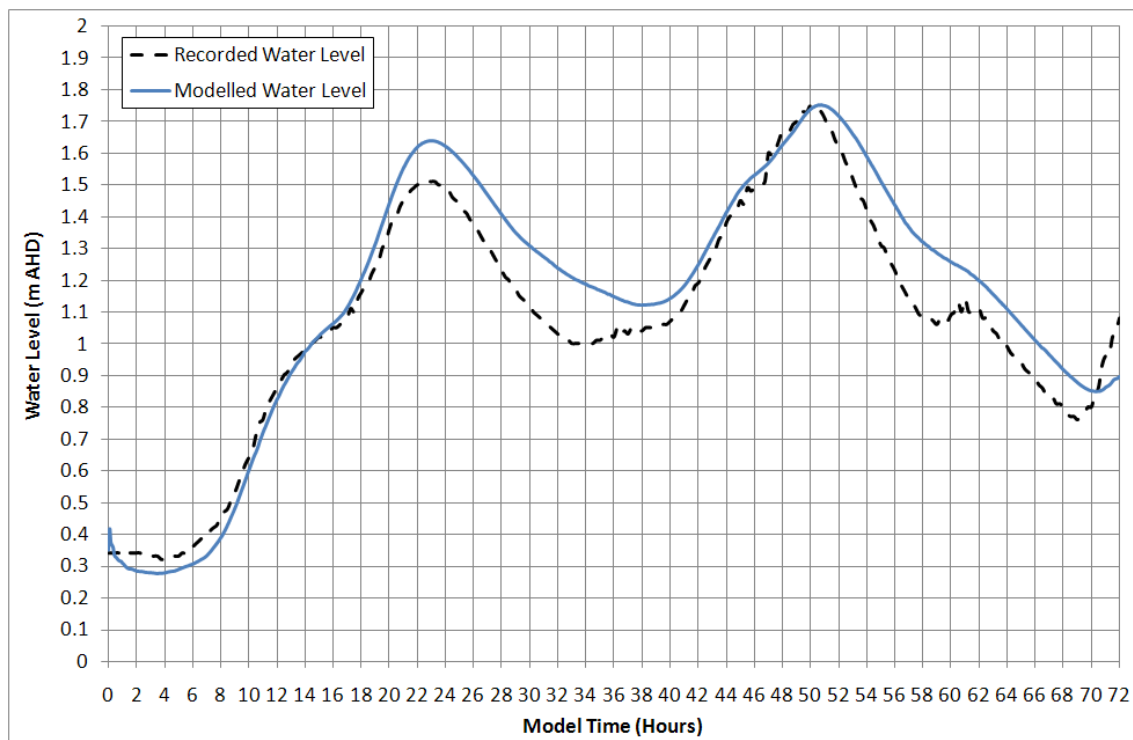
Figure 5-27 Ocean Street Water Level Validation – August 1998
