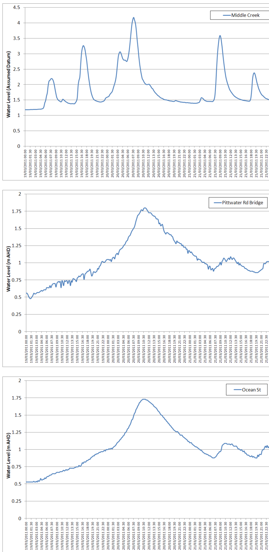
Figure 5-16 March 2011 Recorded Water Levels
