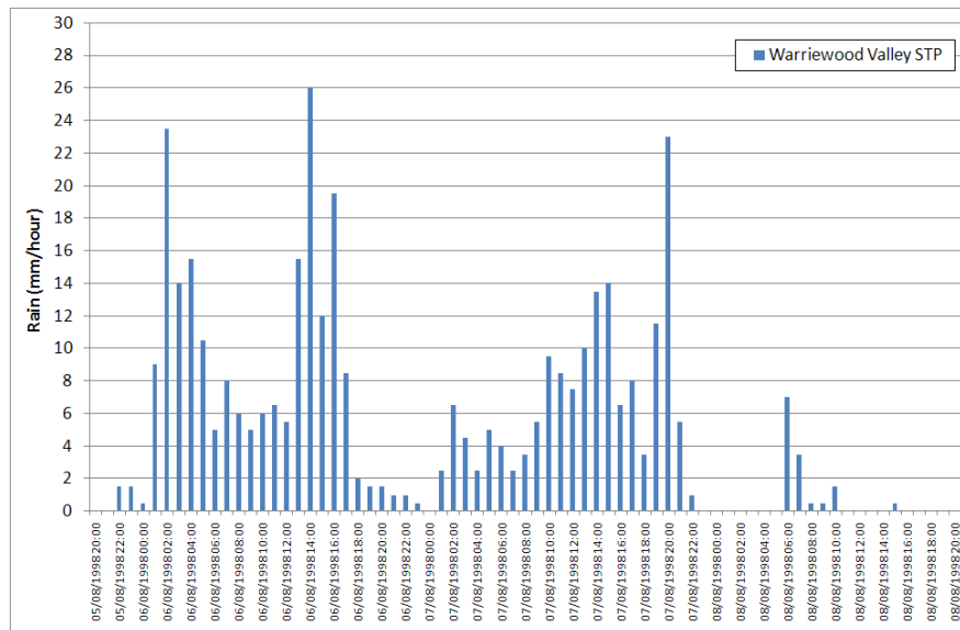
Figure 5-23 August 1998 Recorded Rainfall
