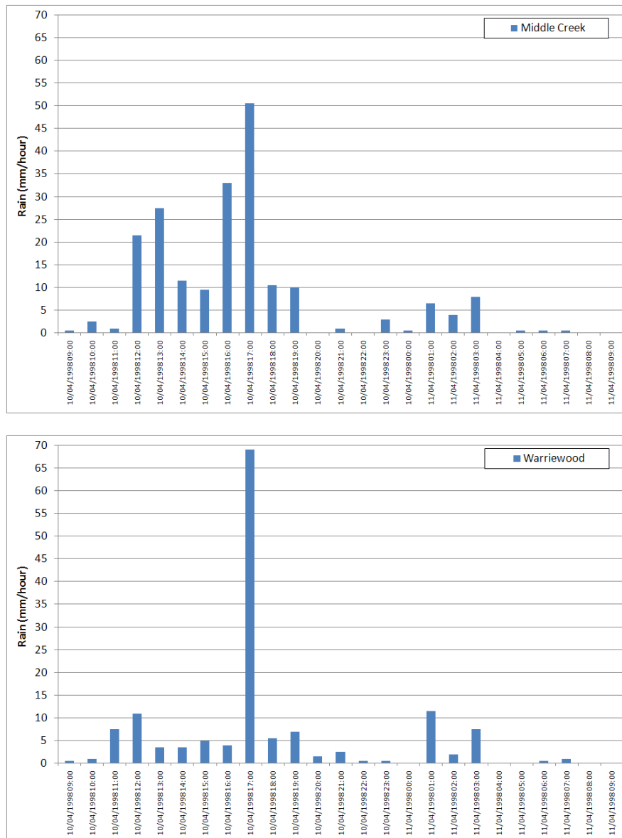
Figure 5-2 April 1998 Recorded Rainfall
