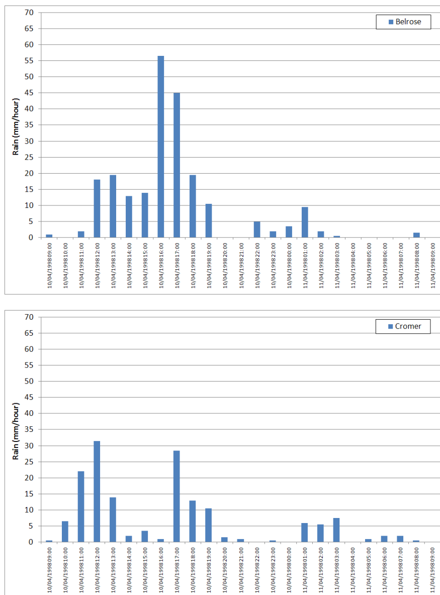
Figure 5-2 April 1998 Recorded Rainfall
