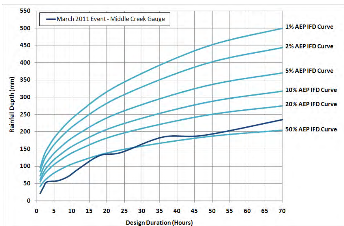
Figure 5-15 Comparison of March 2011 Rainfall with IFD Relationships
