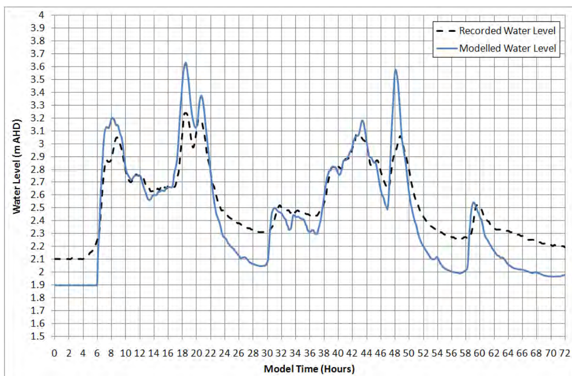
Figure 5-32 Mullet Creek Water Level Validation – August 1998
