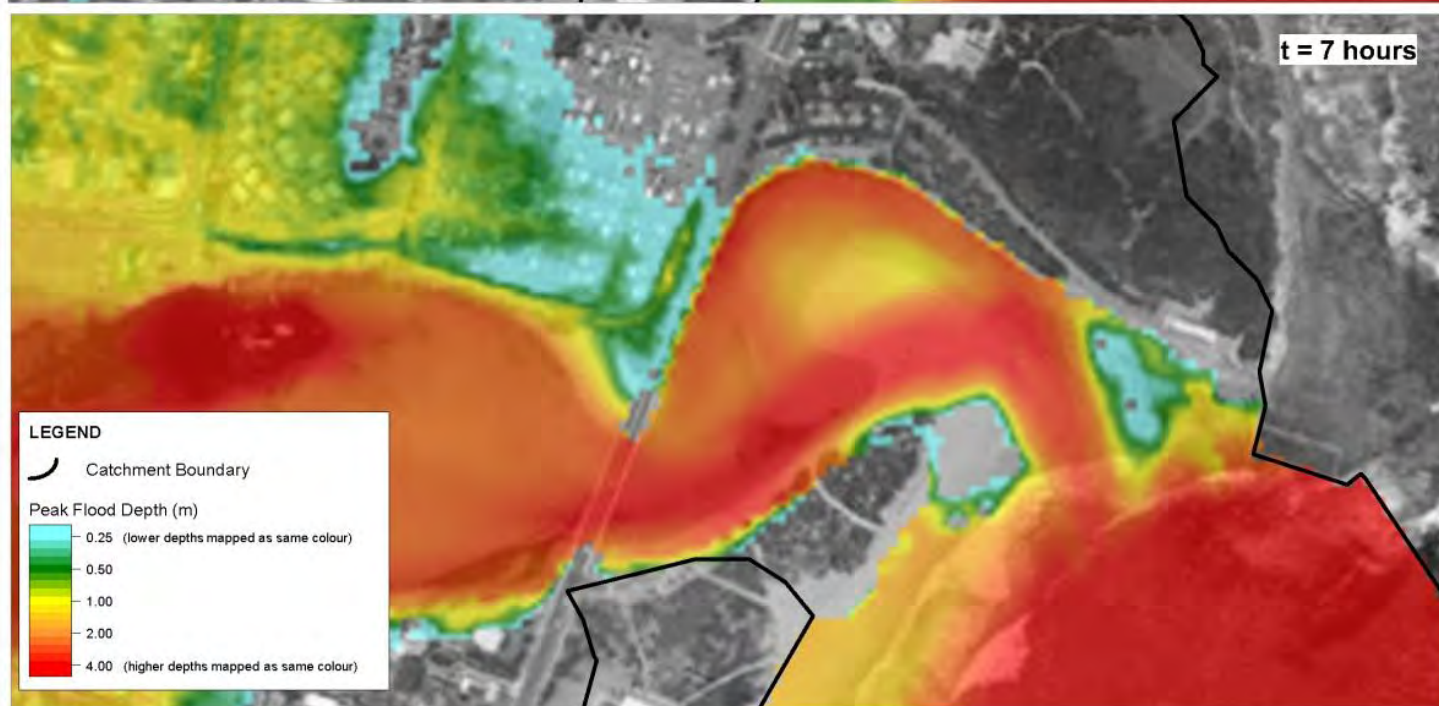
Title: Narrabeen Lagoon Flood Study - Peak Flood Depths: 1% AEP Catchment Derived Event
