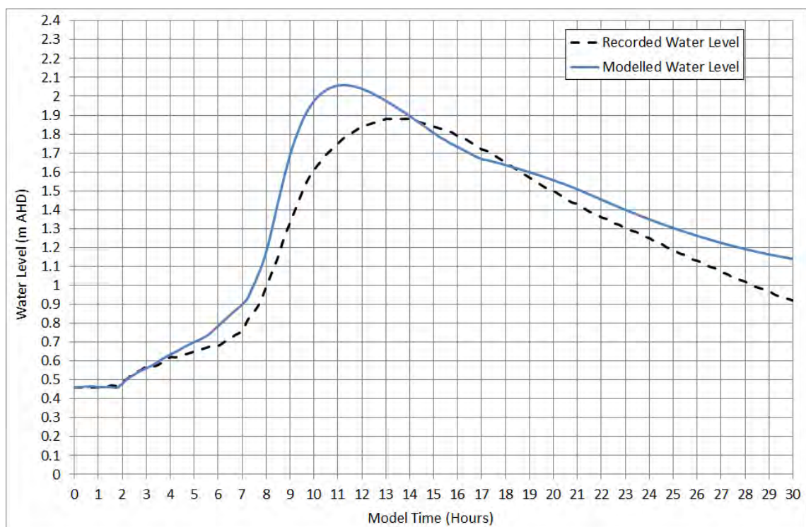
Figure 5-10 Pittwater Road Bridge Water Level Calibration – April 1998
