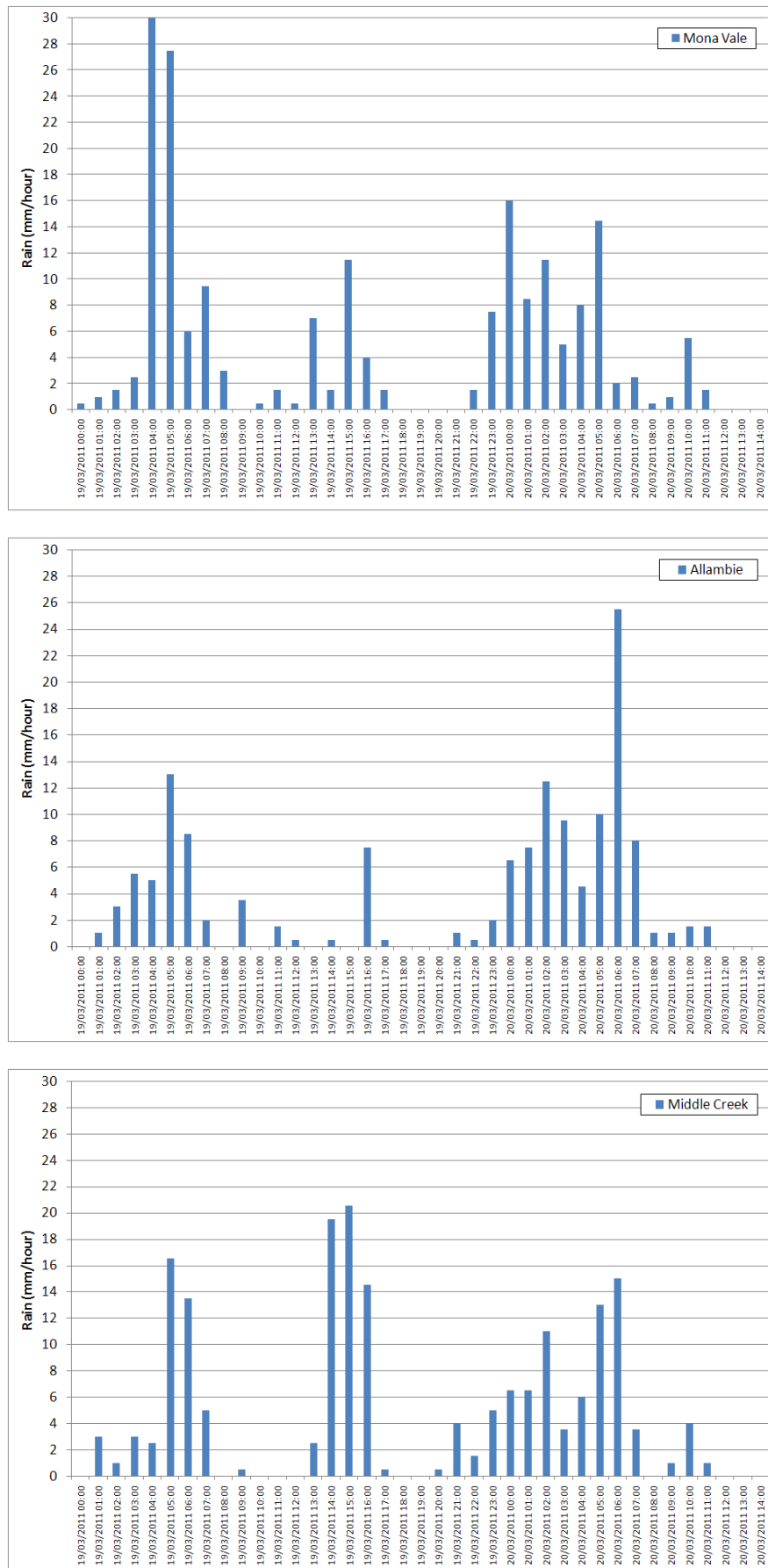
Figure 5-14 March 2011 Recorded Rainfall
