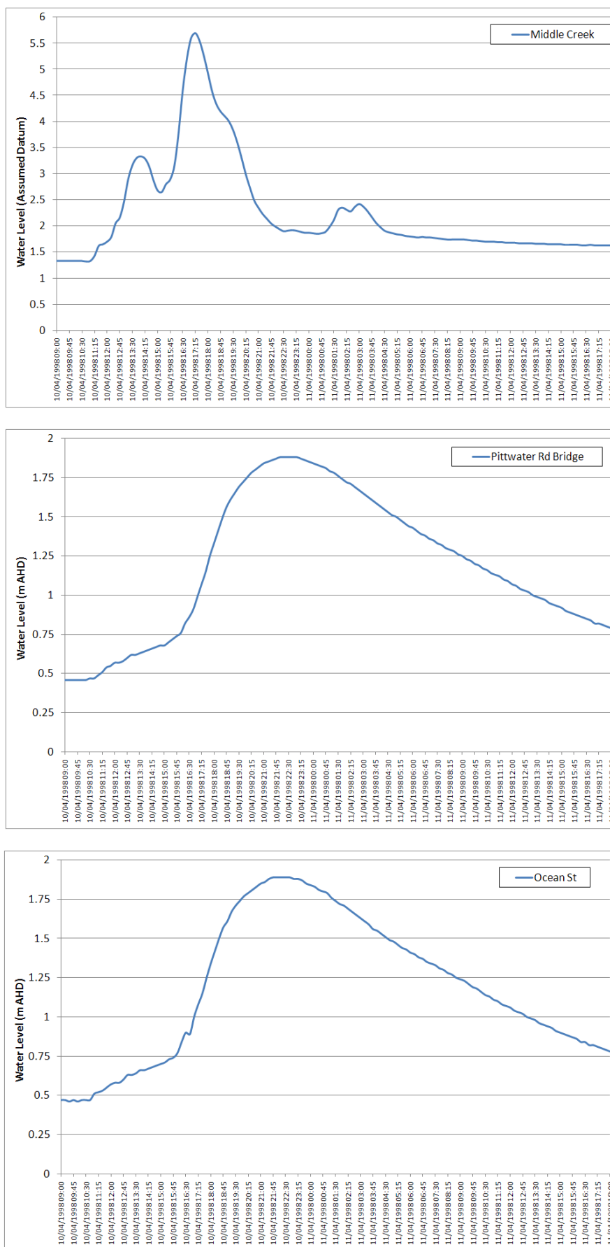
Figure 5-4 April 1998 Recorded Water Levels
