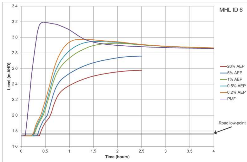
Figure 8.9 – Stage hydrographs, Barrenjoey Road adjacent to Careel Bay ovals
