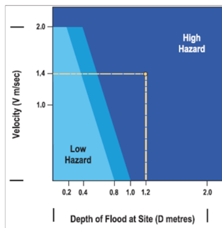
Figure 7.1 – Provisional hydraulic hazard
