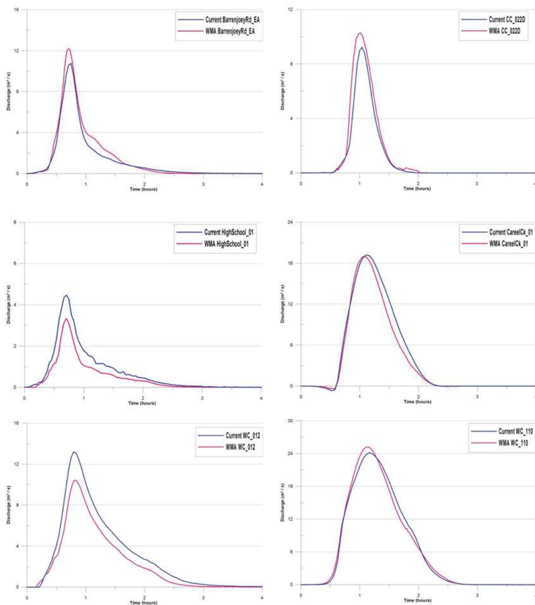
Figure B6 1% AEP 120-minute Event Flow Verification Results
