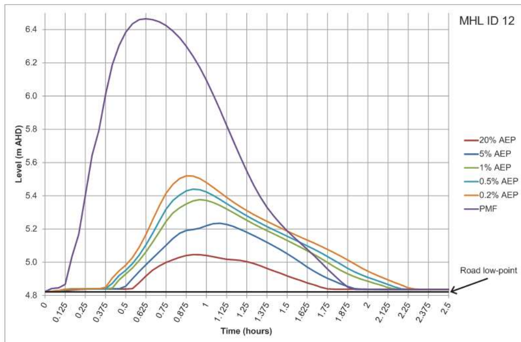
Figure 8.11 – Stage hydrographs, intersection Avalon Parade/Old Barrenjoey Road
