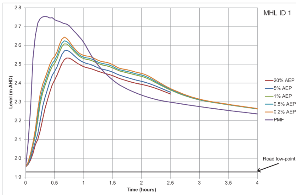
Figure 8.8 – Stage hydrographs, Barrenjoey Road at Palm Beach
