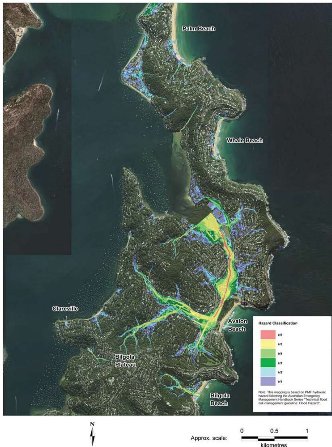
Figure 7.5 – Flood hazard in the PMF
