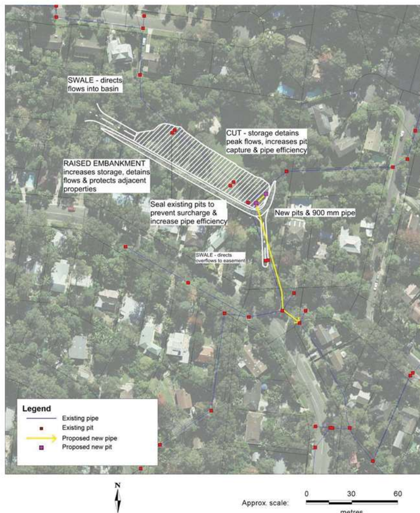
Figure 11.2 – Catalpa Reserve detention basin conceptual layout
