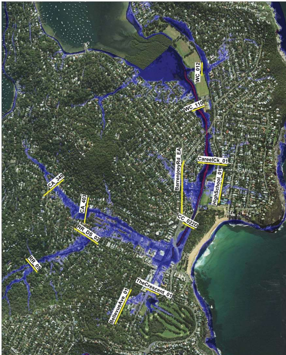
Figure B4 Flow Verification Locations
