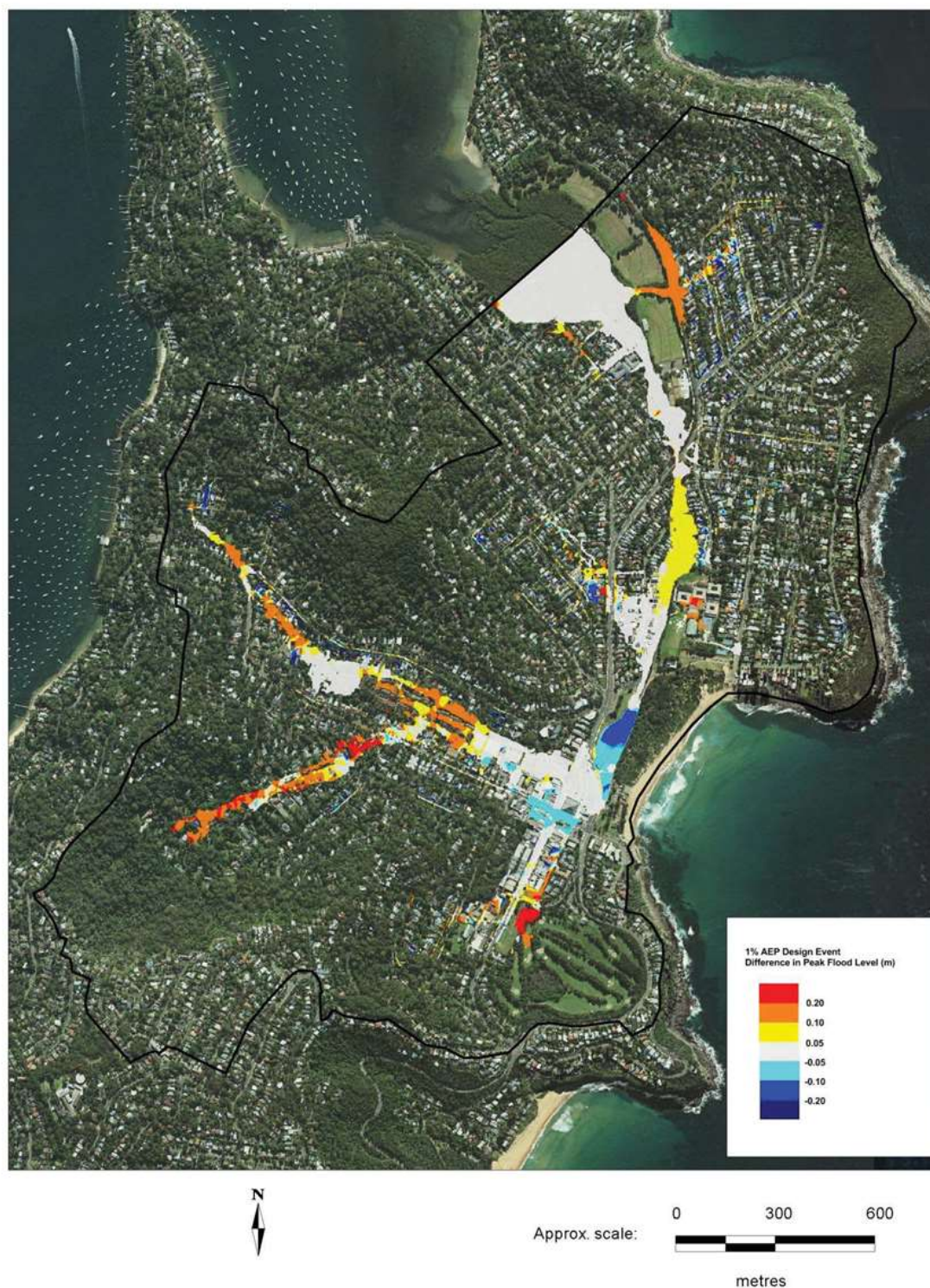
Figure B3 1% AEP Event Flood Level Verification
