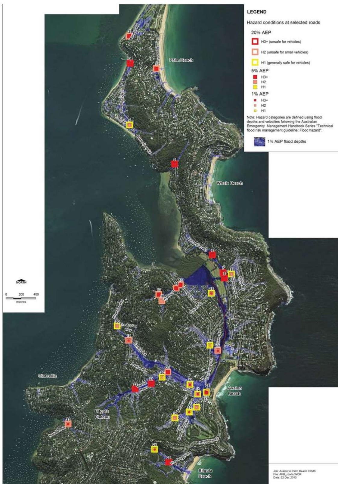
Figure 8.7 – Flood hazard at road low-points
