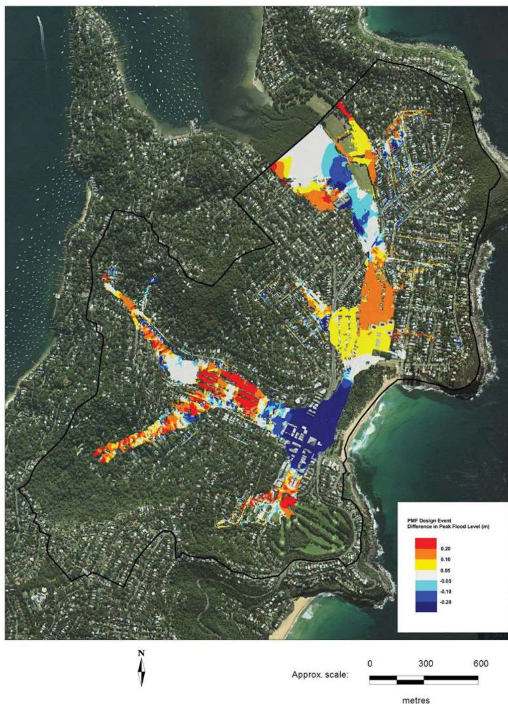
Figure B7 PMF Event Flood Level Verification
