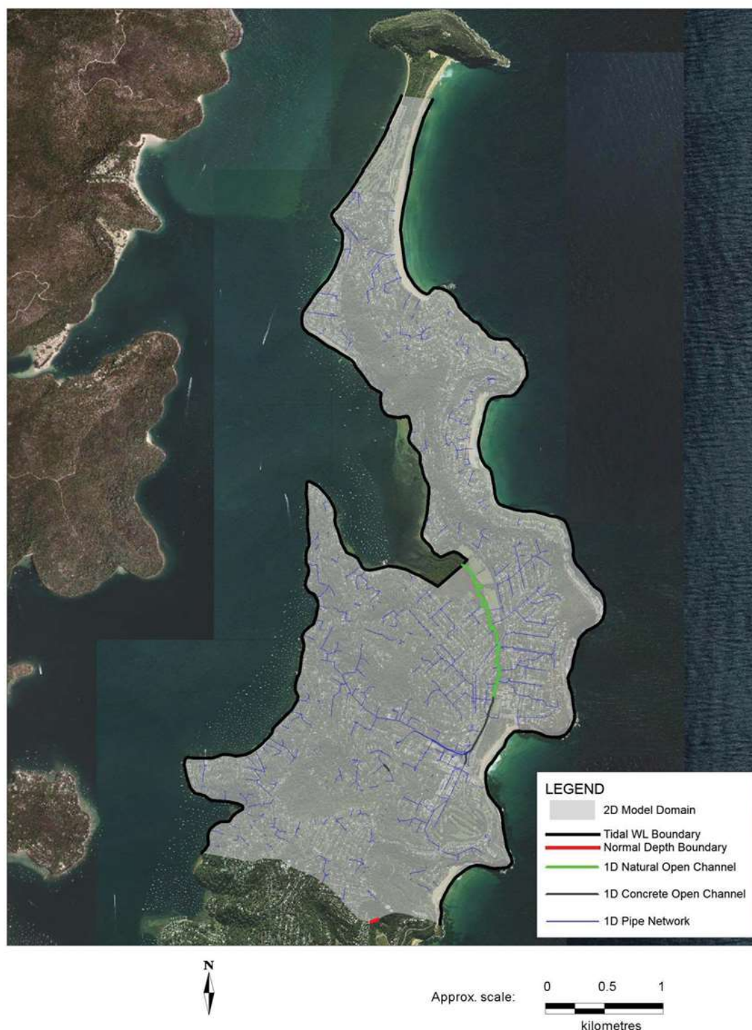
Figure B1 TUFLOW Model Extent and Layout
