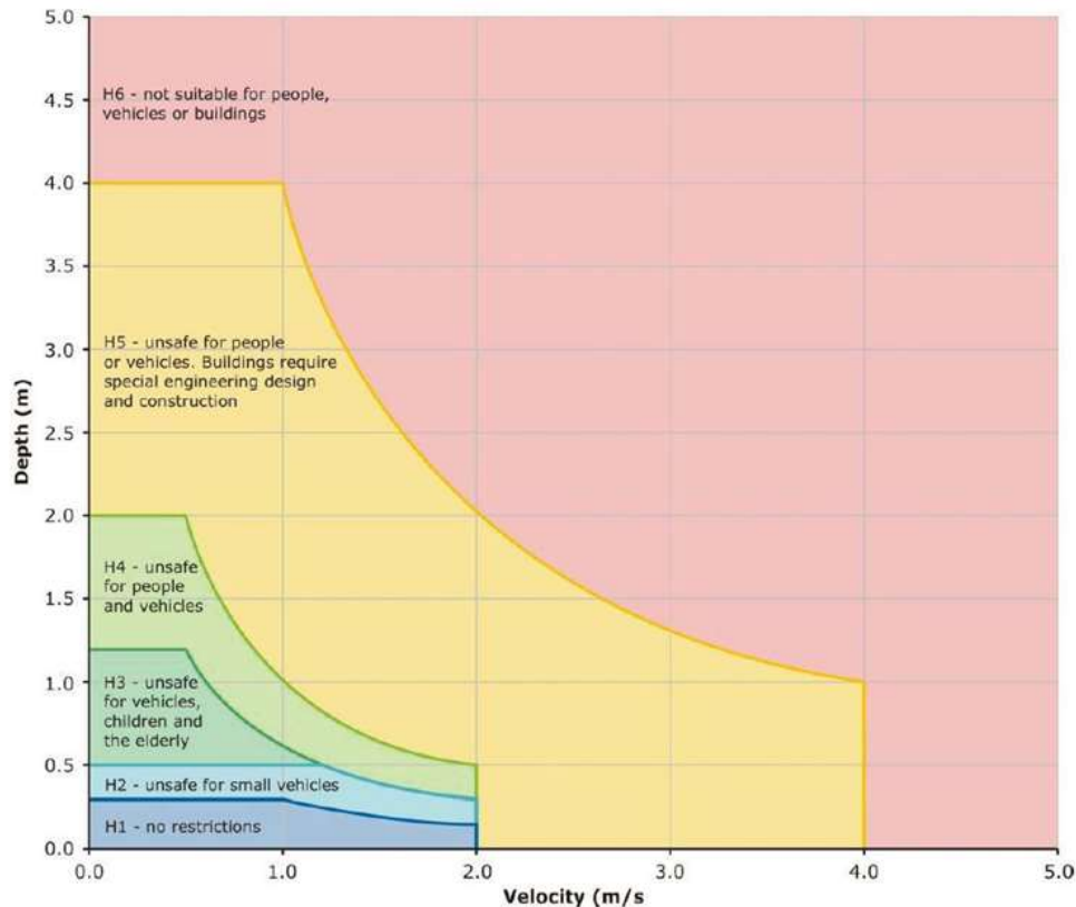
Figure 7.3 – General flood hazard vulnerability curves
