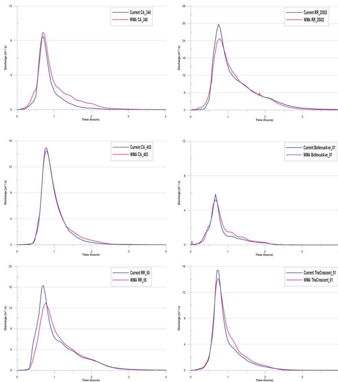
Figure B5 1% AEP 120-minute Event Flow Verification Results
