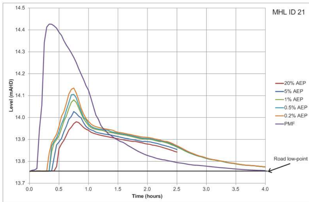
Figure 8.12 – Stage hydrographs, Ruskin Rowe
