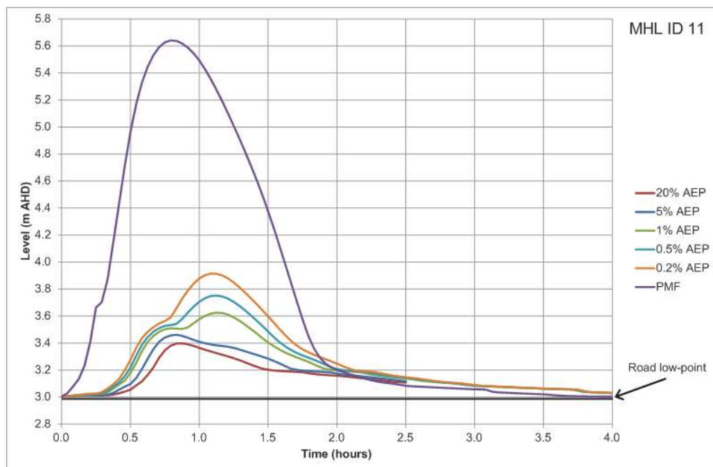
Figure 8.10 – Stage hydrographs, Elaine Avenue
