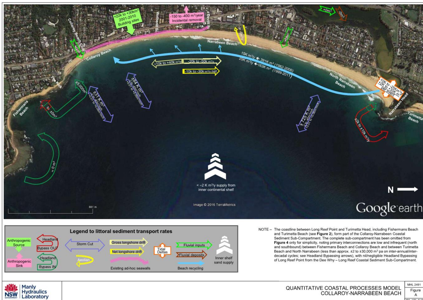
Figure 2-5: Coastal processes model for Collaroy-Narrabeen Beach embayment (Source: Manly Hydraulics Laboratory)
