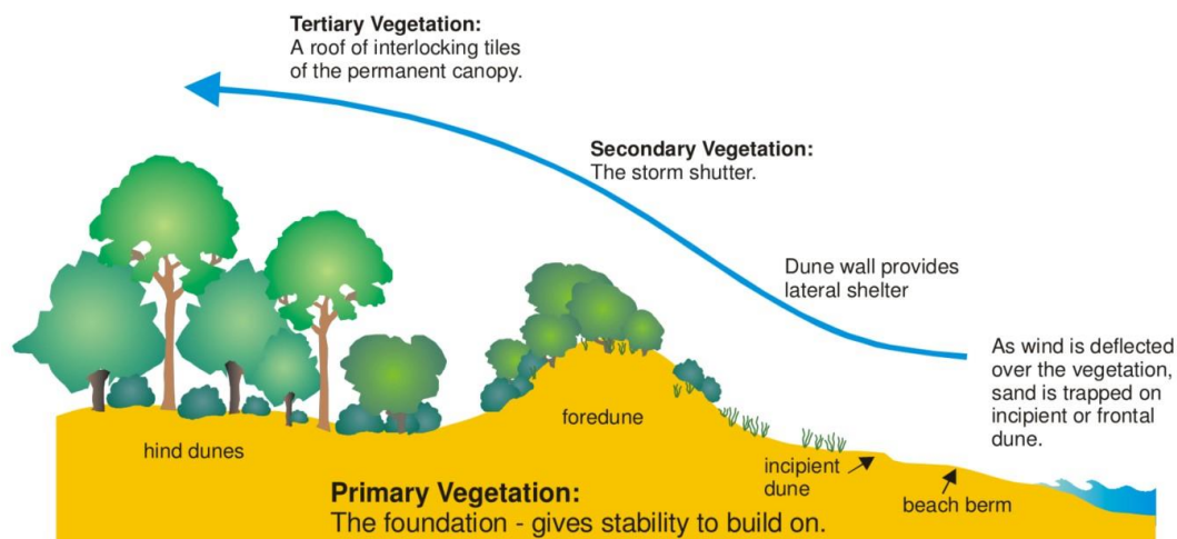
Figure 2-13: Functional model of dune vegetation (DLWC, 2001)
