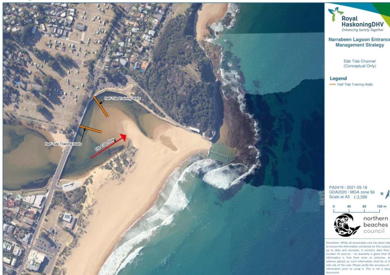
Figure 6-2: Ebb tide channel option conceptual arrangement
