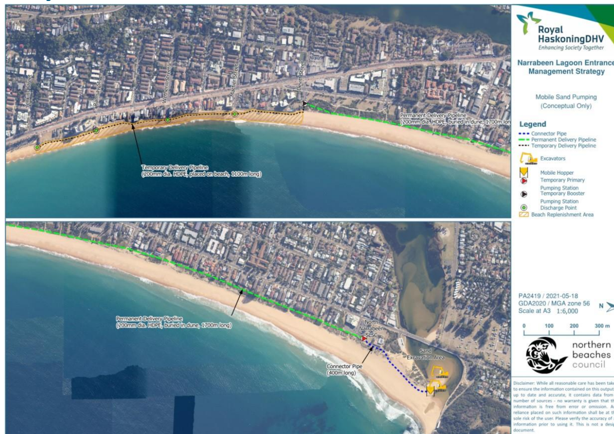
Figure 6-4: Mobile sand pumping option conceptual arrangement
