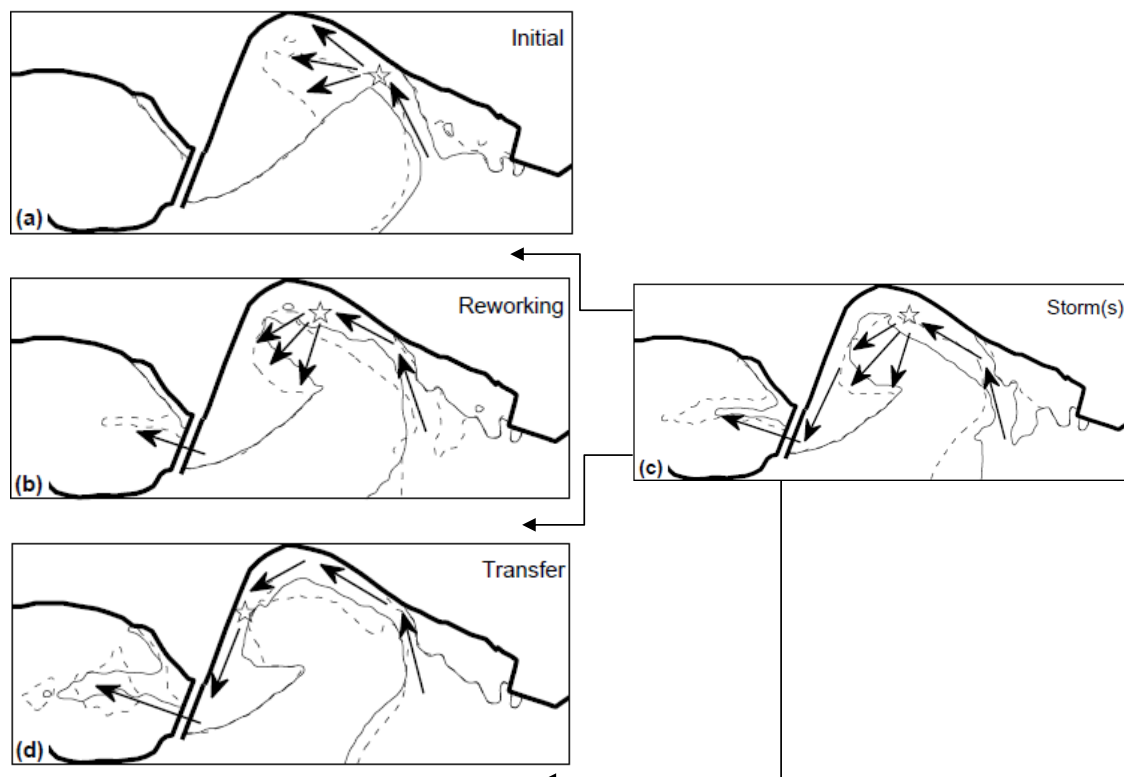
Figure 2-7: Lagoon entrance morphodynamics (Morris, 2010)
