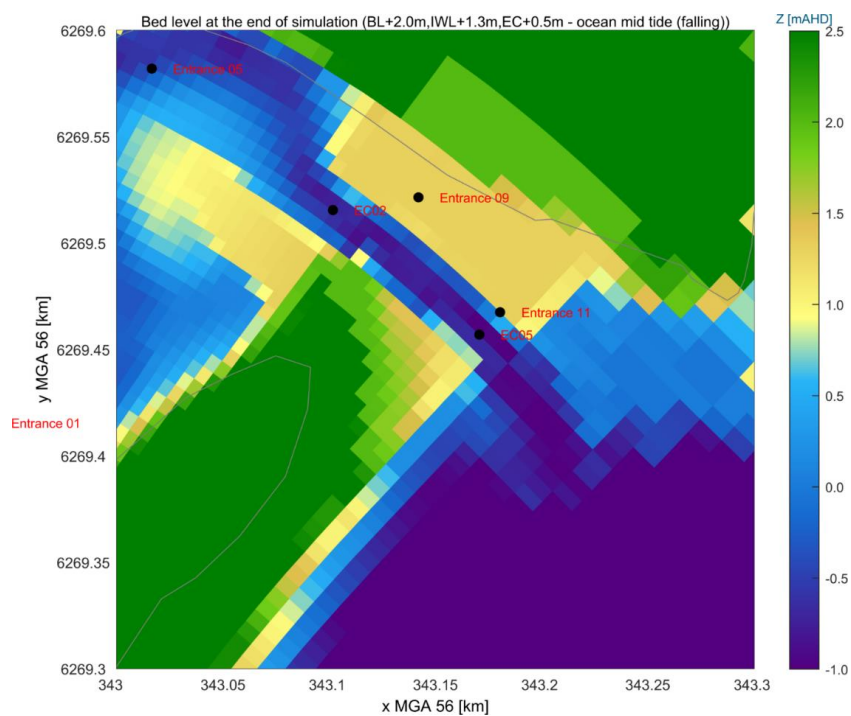
Figure C-2: Delft3D model output locations along breakout channel
