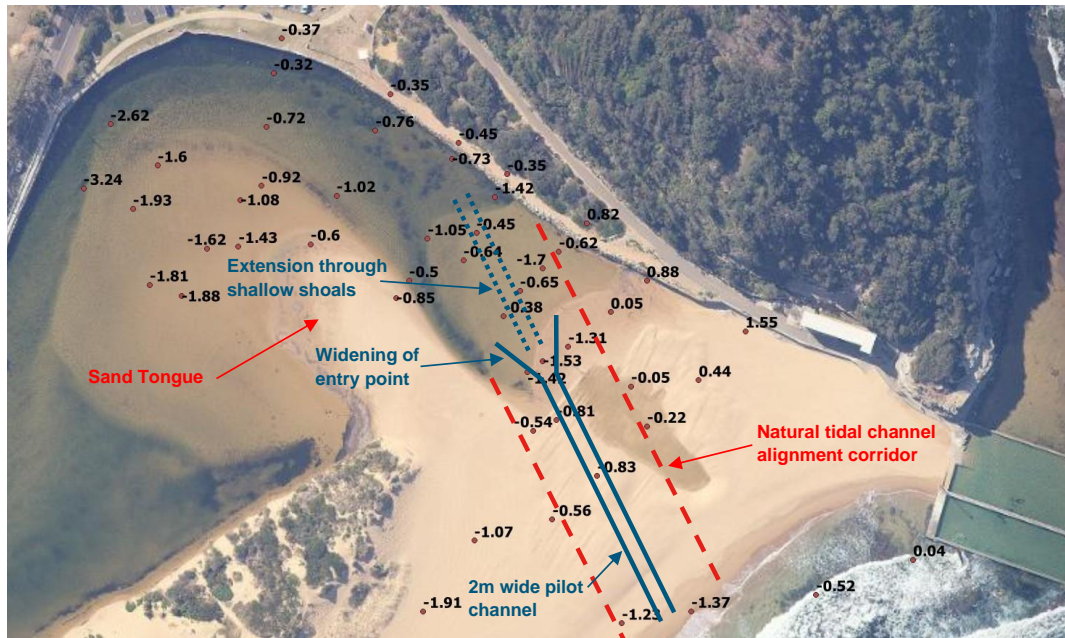
Figure 4-11: Pilot channel recommended arrangement
