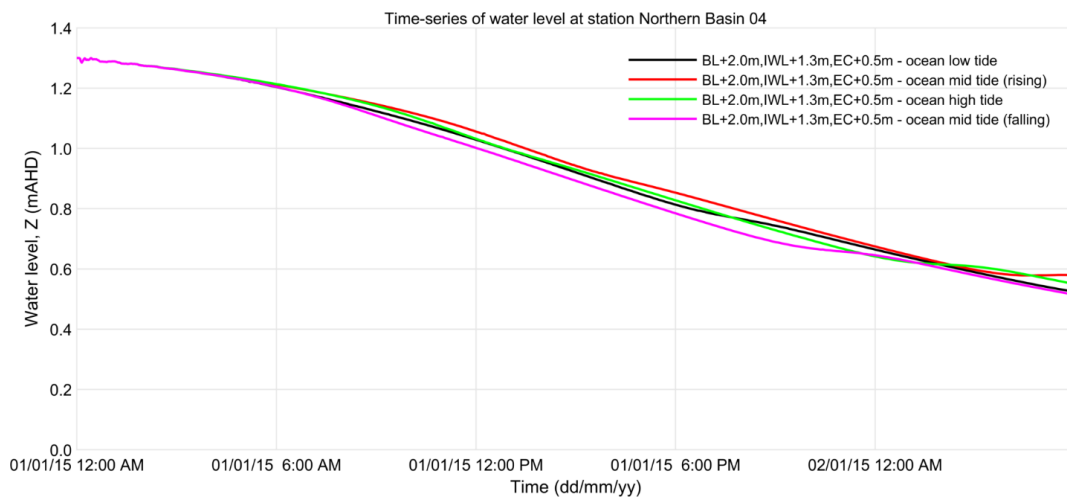
Figure C-4: Lagoon Water Level at Northern Basin 04 – IWL 1.3, BC 0.5
