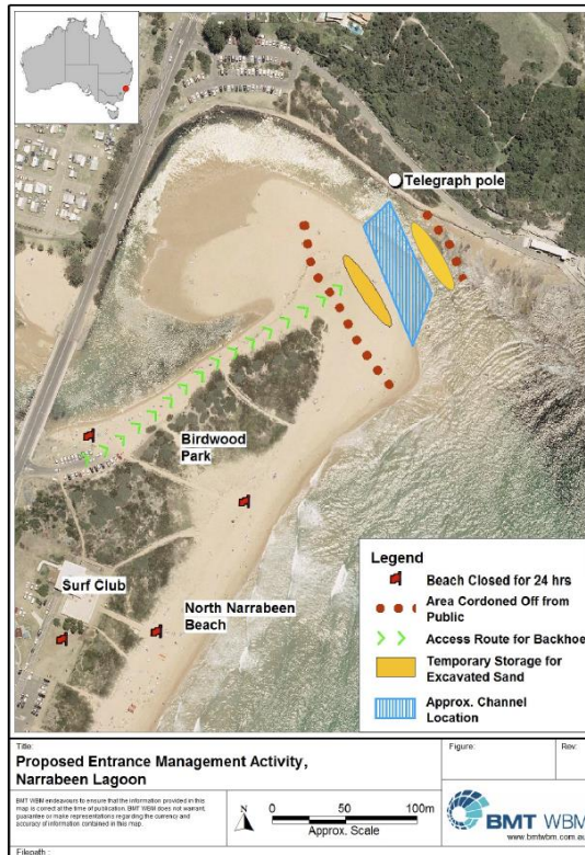
Figure 4-8: Pilot channel alignment in current operating procedure
