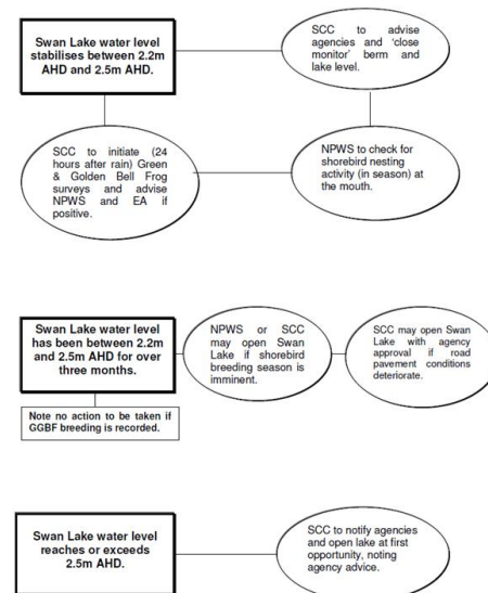
* The decision for opening at lower levels is at the discretion of Council officers Figure 2: Bega River Entrance Management Decision Flow Chart
